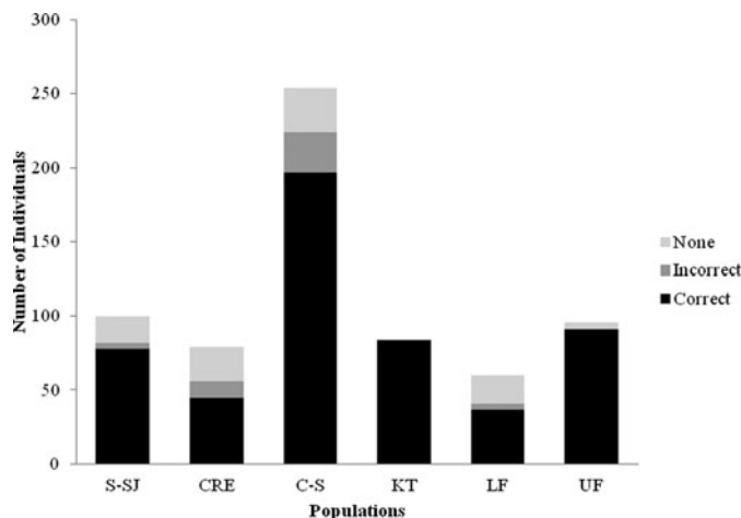
FIGURE 5. Re-allocation of White Sturgeon to populations identified by Structure in the program AFLPOP, MLD = 0.8. See Figure 4 for definition of abbreviations.
