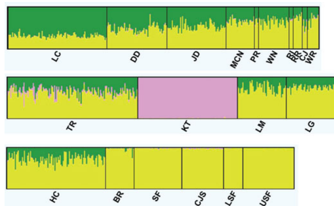
FIGURE 3. Bar histogram output from Structure depicting individual assignments in the Columbia–Snake River drainage. Each bar represents one individual genome, each color represents a genetic cluster identified by Structure, and the proportion of each color in each bar represents the proportional assignment of each individual to each cluster. See Table 1 for population abbreviations. [Figure available online in color.]
