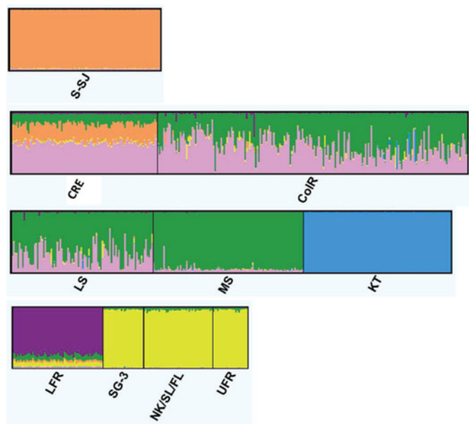
FIGURE 4. Bar histogram outputs from Structure depicting individual assignments in the rangewide data set. Each bar represents one individual genome, each color represents a genetic cluster identified by Structure, and the proportion of each color in each bar represents the proportional assignment of each individual to each cluster. S–SJ = Sacramento–San Joaquin River, CRE = Columbia River estuary, ColR = Columbia River (DD to TR), LS = lower Snake River, MS = middle Snake River, KT = Kootenai River, LFR = lower Fraser River, SG-3 = middle Fraser River, NK/SL/FL = Nechako River/Stuart Lake/Fraser Lake, UFR = upper Fraser River. See Table 1 for more information regarding population abbreviations.
