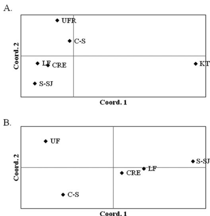
FIGURE 6. Principle coordinates analysis of White Sturgeon populations identified by Structure in range-wide analysis. S–SJ = Sacramento–San Joaquin River, CRE = Columbia River estuary, C–S = The Dalles to Transboundary Reach of Columbia River, lower Snake River, and middle Snake River, KT = Kootenai River, LF = lower Fraser River, and UF = upper Fraser River. (A) PCA conducted with the Kootenai River population. (B) PCA excluding the Kootenai River population.
