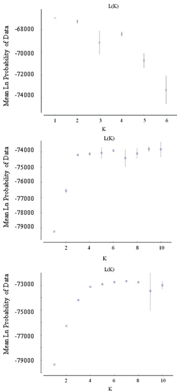
FIGURE 2. Mean \ln \Pr(X|K) values for Structure examination of population structure (A) within the Sacramento–San Joaquin River system, (B) within the Columbia–Snake River drainage, and (C) among drainages across the species’ range. Vertical lines denote SD.
