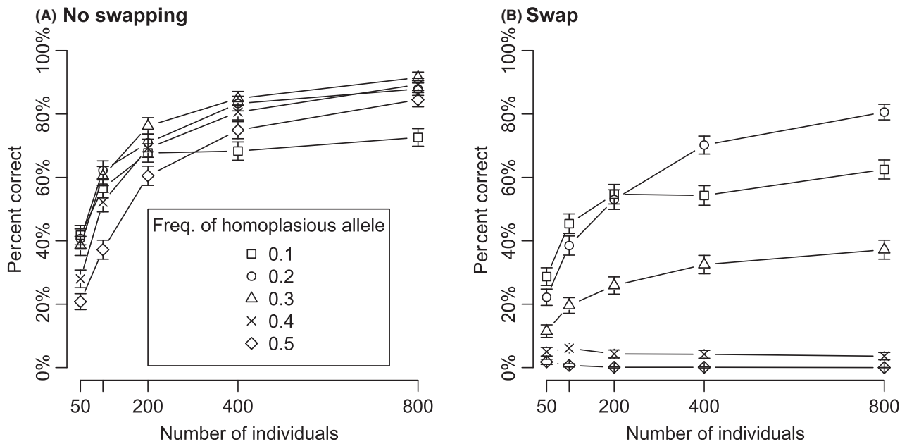
Fig. 4 Percentages of simulated data sets with correct allele assignments when homoplasious alleles are present. Whiskers indicate 95% confidence intervals. The y -axis indicates the percentage of data sets for which allele assignments were completely correct. Allotetraploid data sets were simulated with one pair of homoplasious alleles (alleles from two different isoloci, but with identical amplicon size) for each locus. The frequency of homoplasious alleles was identical at both isoloci in each data set and was set at five different levels (0.1 through 0.5). Five different sample sizes were tested (50, 100, 200, 400 and 800). For each homoplasious allele frequency and sample size, 1000 data sets were simulated. Allele assignments were made using two methods: k -means + UPGMA (A; swap = FALSE) and k -means + UPGMA + swap (B; swap = TRUE); plus an algorithm in the function testAlGroups that identifies the alleles most likely to be homoplasious, and assigns alleles as homoplasious until all genotypes are consistent with allele assignments.
