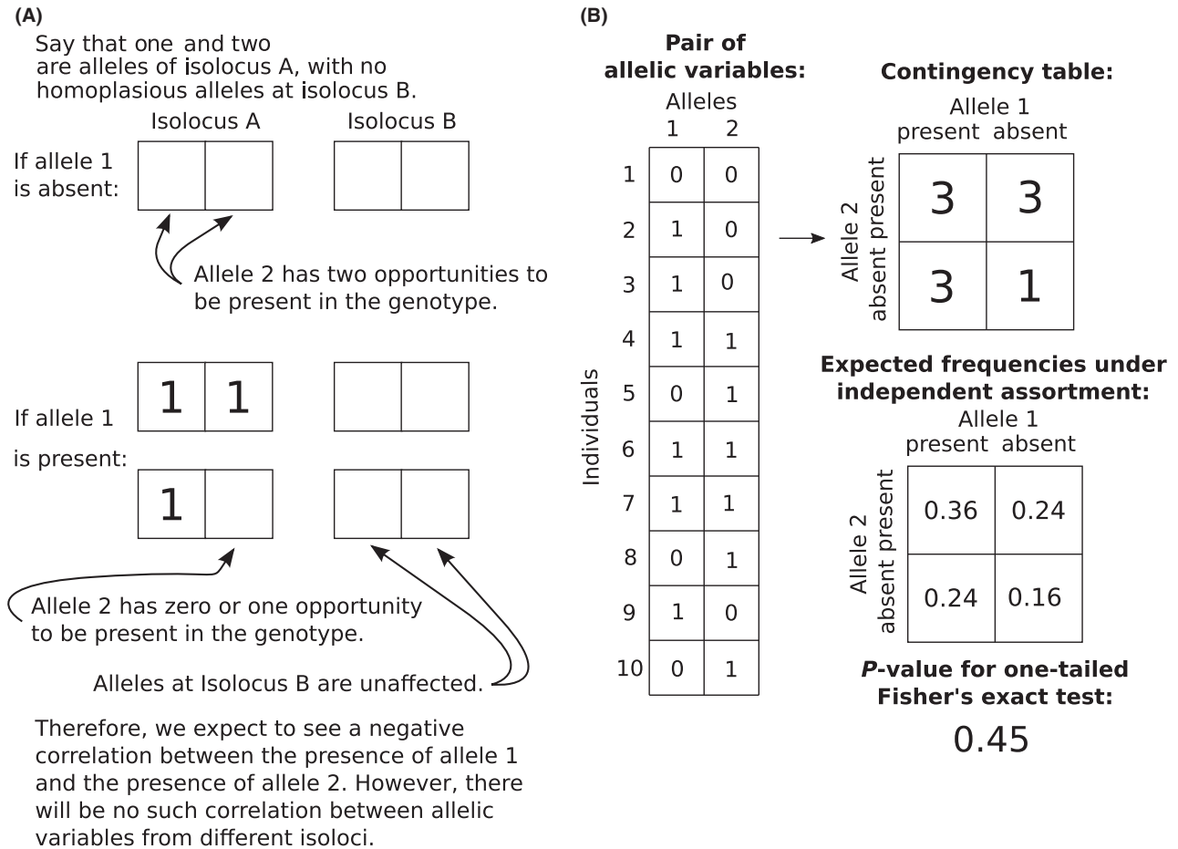
Fig. 1 Negative correlation between two allelic variables at a locus. (A) Qualitative reasoning for the expectation of negative correlation between two allelic variables at the same isolocus. (B) Use of Fisher's exact test to identify negative correlation between a pair of allelic variables. Ten individuals are shown for the sake of illustration, but an ideal data set would have 100 or more individuals. In the allelic variables, the presence of an allele in an individual is indicated by 1, and the absence is indicated by 0.
