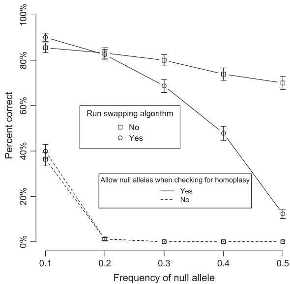
Fig. 5 Percentages of simulated data sets with correct allele assignments when one isolocus has a null allele. Whiskers indicate 95% confidence intervals. The y -axis indicates the percentage of data sets for which allele assignments were completely correct. Allotetraploid data sets were simulated, and frequency of the null allele was set at one of five levels ( x -axis). A total of 1000 data sets were simulated at each null allele frequency. Two parameters for testAlGroups were adjusted: swap at values of false or true (corresponding to the methods k-means + UPGMA and k-means + UPGMA + swap , respectively); and null.weight at values of zero (null alleles are allowed when checking for evidence of homoplasia) and 0.5 (genotypes lacking alleles belonging to a given isolocus are taken as evidence that their other alleles are homoplasious).
