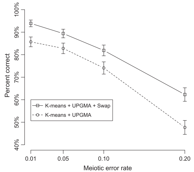
Fig. 6 Percentages of simulated data sets with correct allele assignments when meiotic error causes compensated aneuploidy. Whiskers indicate 95% confidence intervals. The y -axis indicates the percentage of data sets for which allele assignments were completely correct. Meiotic error was simulated in the simAllopolypoly function on a per-gamete basis, with each error causing an allele from one isolocus to be substituted with an allele from the other isolocus. Each data set was otherwise simulated for an allotetraploid organism with 100 individuals. Meiotic error rate, as shown in the x -axis, was controlled using the meiotic.error.rate argument of simAllopolypoly . For each error rate, 1000 data sets were simulated. For the testAlGroups function, the tolerance argument was set to 1 to prevent the function from checking for homoplasia, and swap was set to false or true (corresponding to the methods k-means + UPGMA and k-means + UPGMA + swap , respectively). Each data set was tested for both values of swap .
