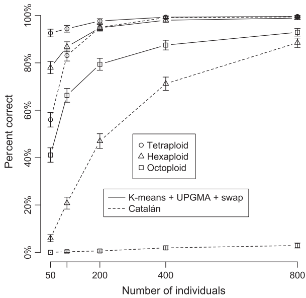
Fig. 3 Accuracy of allele assignments with different sample sizes. For each ploidy and sample size, 1000 simulations were performed. Octoploids were simulated with two tetraploid genomes. Whiskers indicate 95% confidence intervals. ‘Swap’ indicates that testAlGroups was used with swap = TRUE . The y -axis indicates the percentage of data sets for which allele assignments were completely correct.
